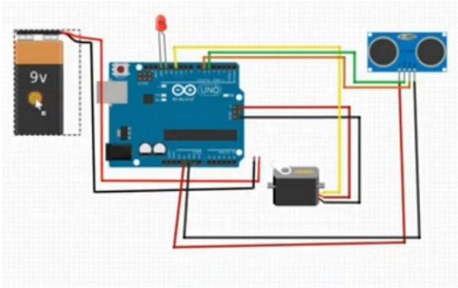
Figure: Circuit Diagram (source: https://www.youtube.com/watch?v=7UStiMiKlTI )
